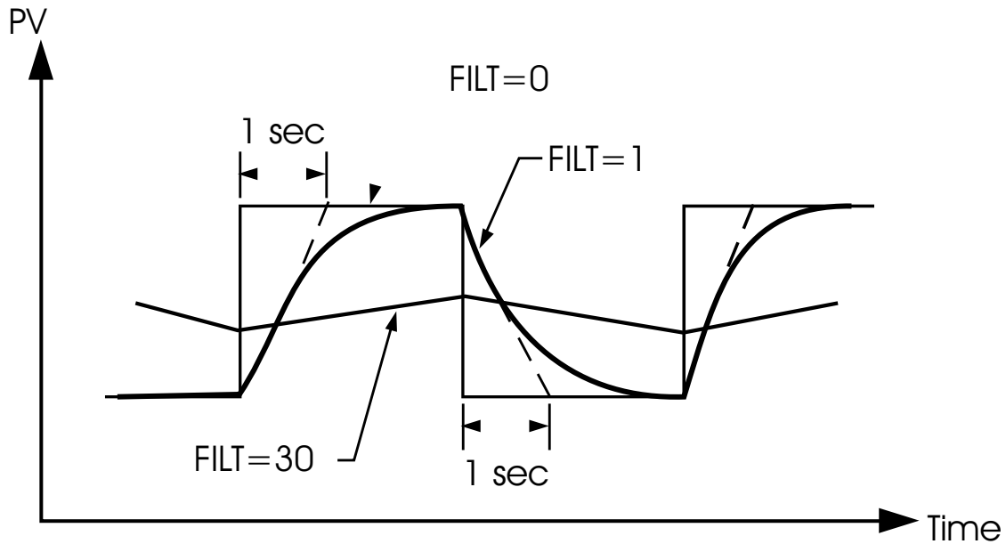
Figure 3.8 Filter Characteristics
