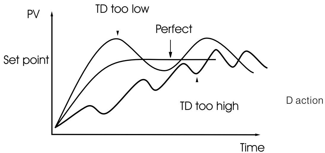
Figure 3.9 Effects of PID Adjustment
