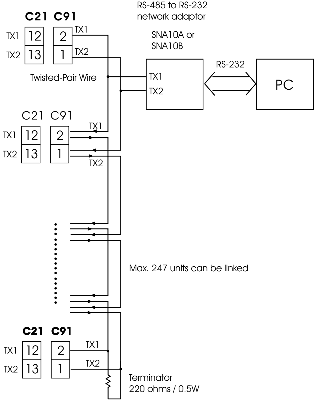
Figure 2.21 RS-485 Wiring
